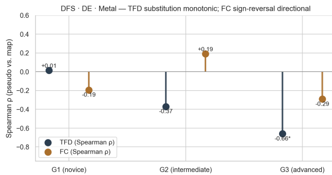
Fig. 3: DFS DE Metal: Spearman \rho between pseudocode and map for TFD (lead) and FC (secondary). The TFD column moves from 0 to -0.66 ; the FC column shows the directional sign reversal noted in the paper. Asterisk marks p < .05 .
