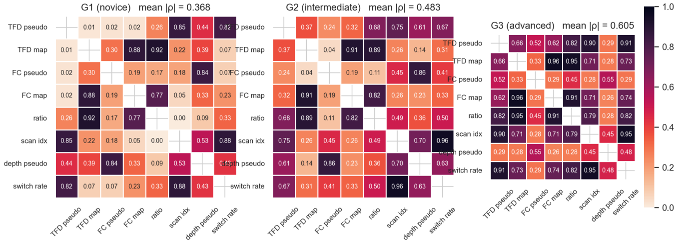
Fig. 4: Pairwise |p| between eight gaze metrics on the DFS DE Metal stimulus. By group, per metric. Mean |p| rises from .368 (G1) to .483 (G2) to .605 (G3); cells in the G3 panel grow darker, showing tighter inter-metric coupling at higher expertise.
